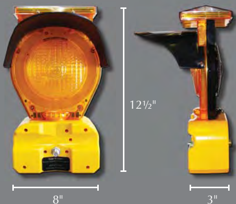
WLSBL006Y Amber Barricade Light TYPE B Solar with orange case
