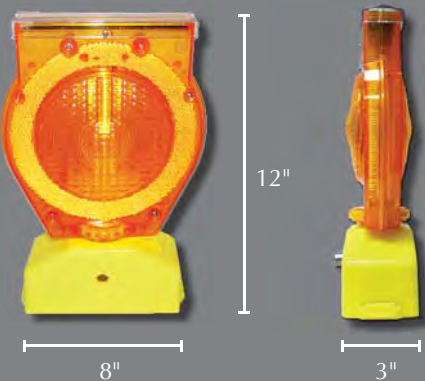
WLDFO02Y Amber Barricade Light TYPE C Solar with yellow case
