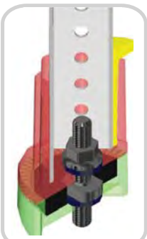
PASBH5840Z Shear Bolt Assembly
